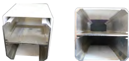
Gate post stiffeners and surface mounts
